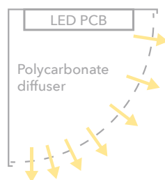
Cross section showing light distribution
