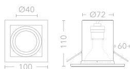
CUT OUT 90x95mm
