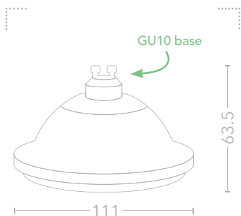
ES111 lamp ( not included.)
